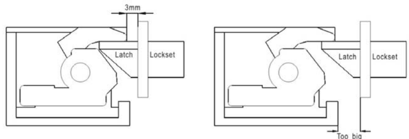
ALLOWABLE LATCH CAVITY
