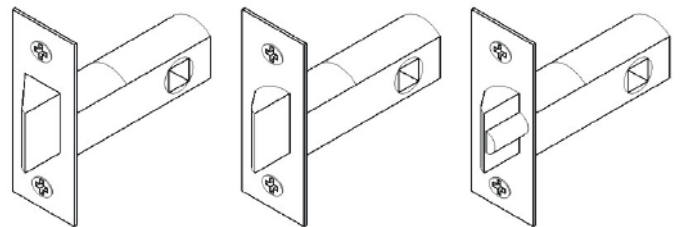
LATCH TYPE
